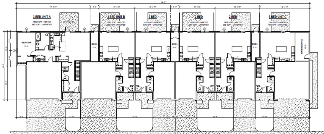
2 SECOND FLOOR PLAN
