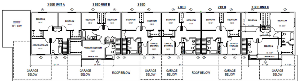
2 SECOND FLOOR PLAN
