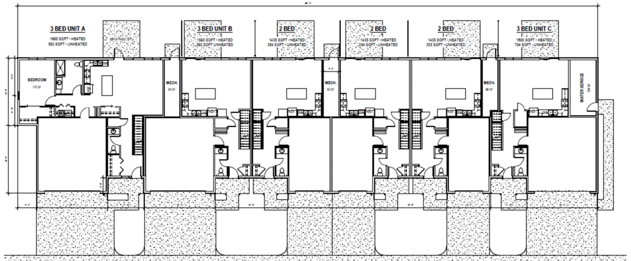
② SECOND FLOOR PLAN 152' x 112'
